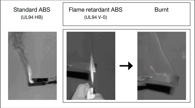
Fig. 3 Flame retardant case (Self-extinguish phenomenon)
