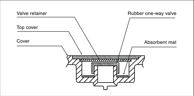
Example of Valve Construction
