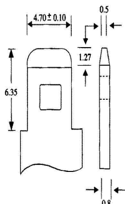
FASTON 187 SERIES
